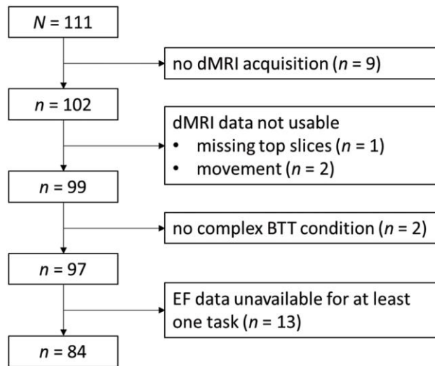
Supplementary Figure 1. Flow chart for selection of observations. Note. Only complete datasets were retained for the current analyses. Please see Seer et al. (2021) for details regarding the availability of EF data. BTT = bimanual tracking task, dMRI = diffusion magnetic resonance imaging, EF = executive functioning.
