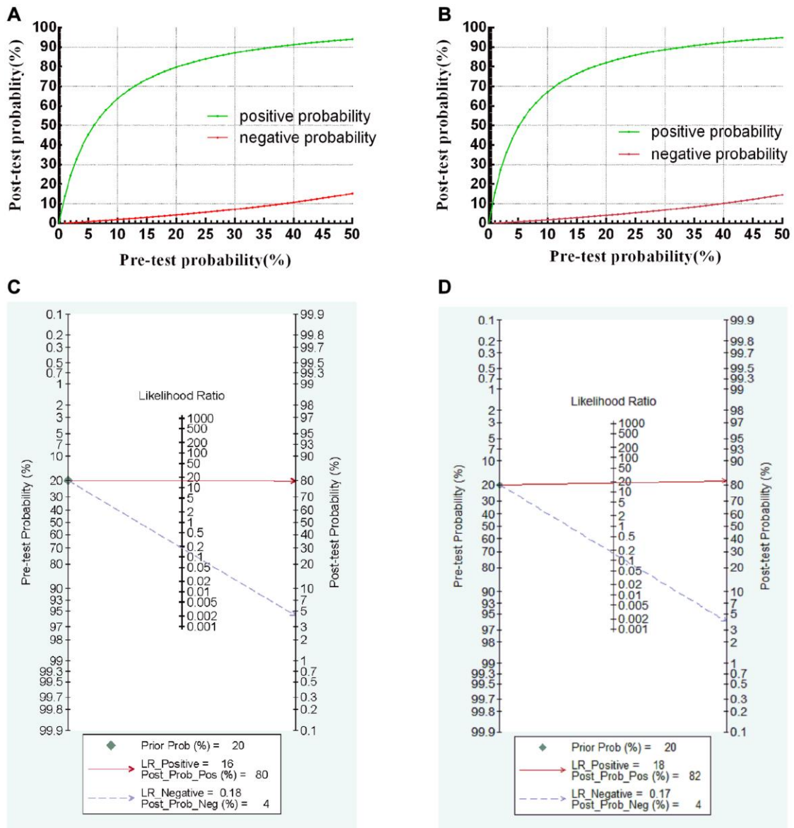
Supplementary Figure 5. Line charts and Fagan’s plots indicating diagnostic probability. (A) diagnostic probability line chart of total microRNAs; (B) diagnostic probability line chart of single miR-371a-3p; (C) Fagan’s plot based on the TGCT pre-test probability of 20% for total microRNAs; (D) Fagan’s plot based on the TGCT pre-test probability of 20% for single miR-371a-3p.
