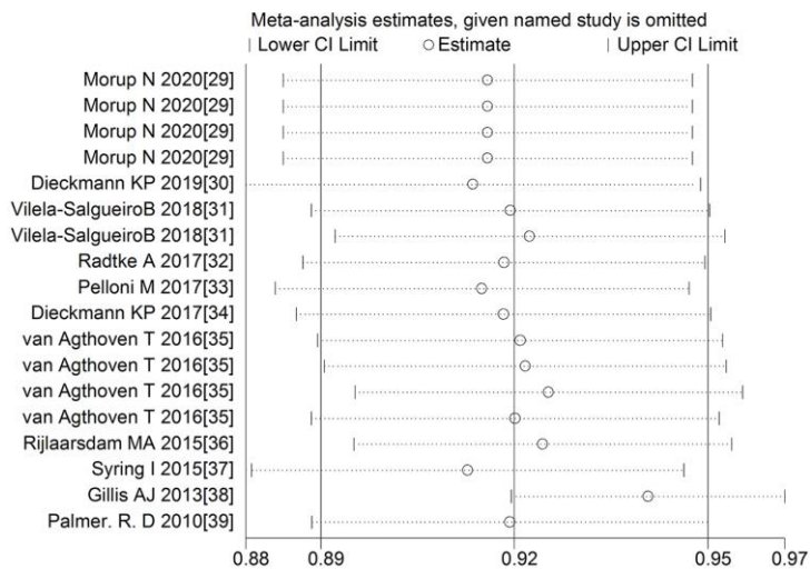
Supplementary Figure 2. Sensitivity analysis of the included studies.
