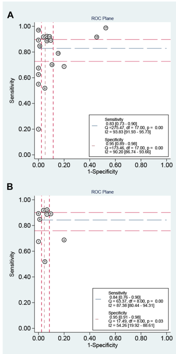
Supplementary Figure 1. ROC plane of the included studies. (A) ROC plane of total microRNAs; (B) ROC plane of single miR-371-3p.
