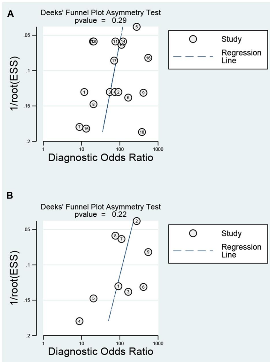
Supplementary Figure 3. Estimation of the publication bias by Deeks' funnel plots. (A) Deeks' funnel plots of total microRNAs ( P = 0.29 ); (B) Deeks' funnel plots of single miR-371a-3p ( P = 0.22 ).
